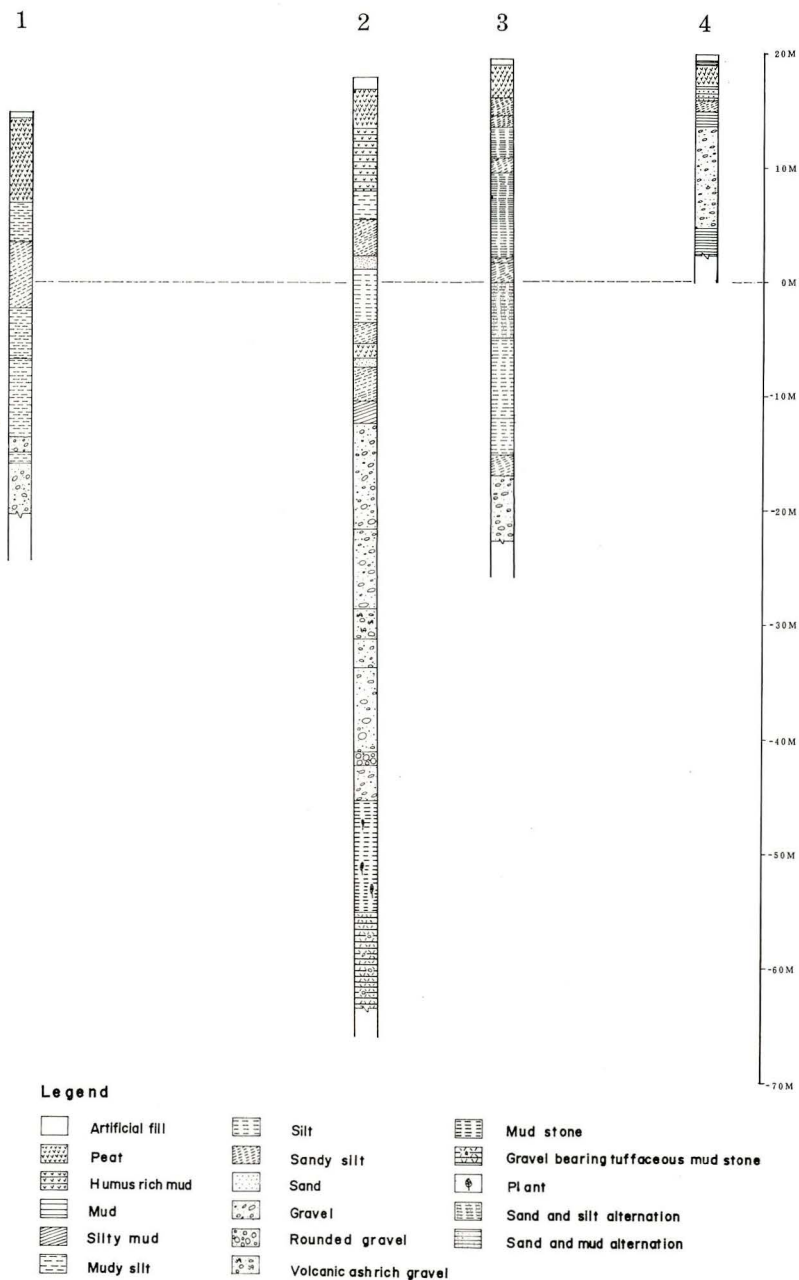
Fig. 3. Columnar section of the back swamp.
